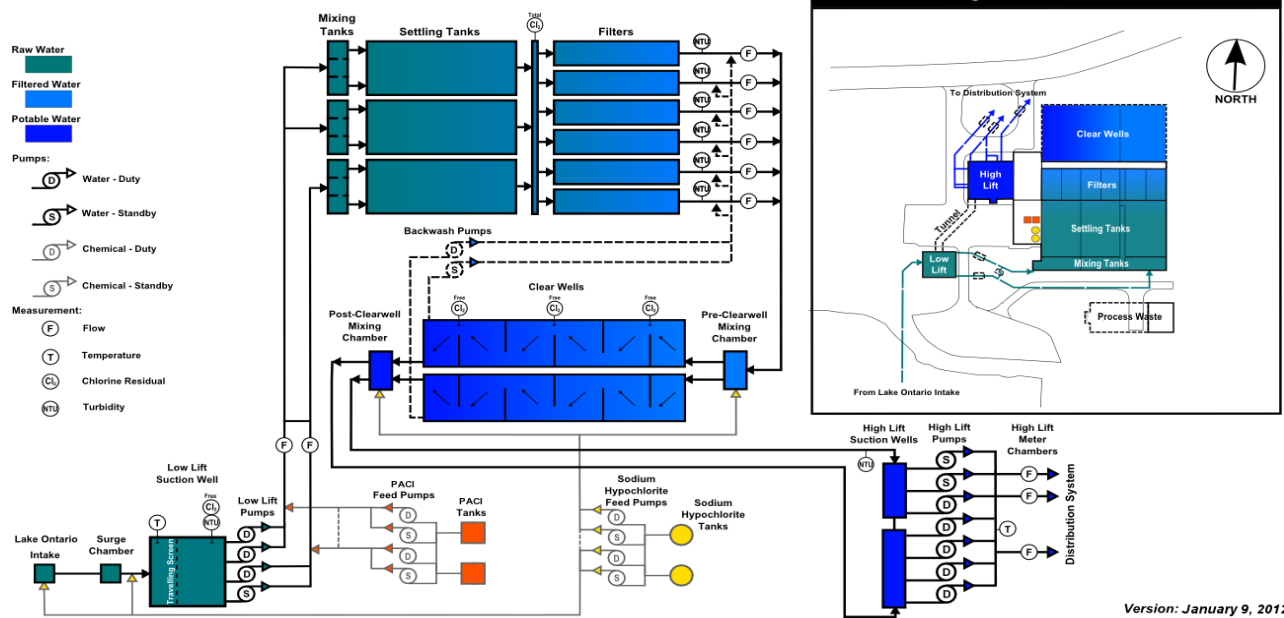
KINGSTON DRINKING WATER SYSTEM - DISTRIBUTION PROCESS FLOW
